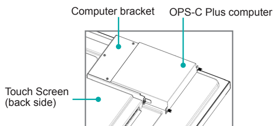
Schematic diagram after the assembly of the OPS-C Plus computer
